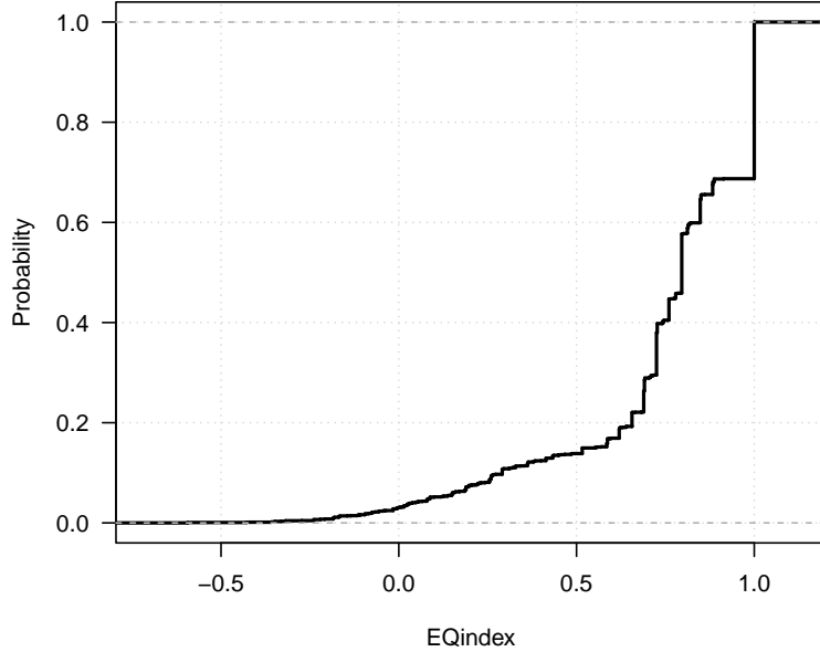
Figure 7: The empirical distribution of the quality-of-life index (EQ-5D) in the pooled dataset of burn patients.
